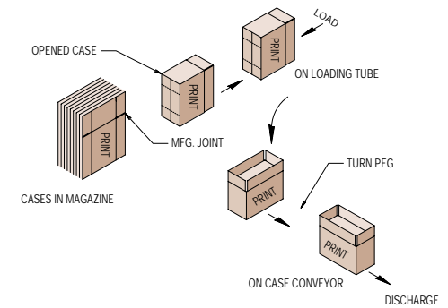
Vertical Case Opening Sequence
