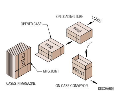
Horizontal Case Opening Sequence
