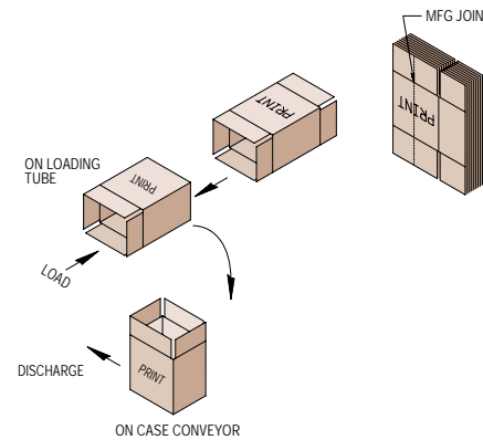
Vertical Case Opening Sequence (CP450)
