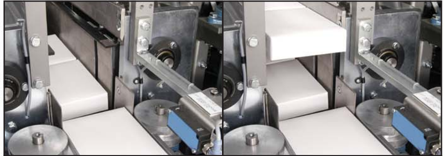
First layer of product, from infeed conveyor, accumulates in a metered quantity inside the AS 100 stacker
